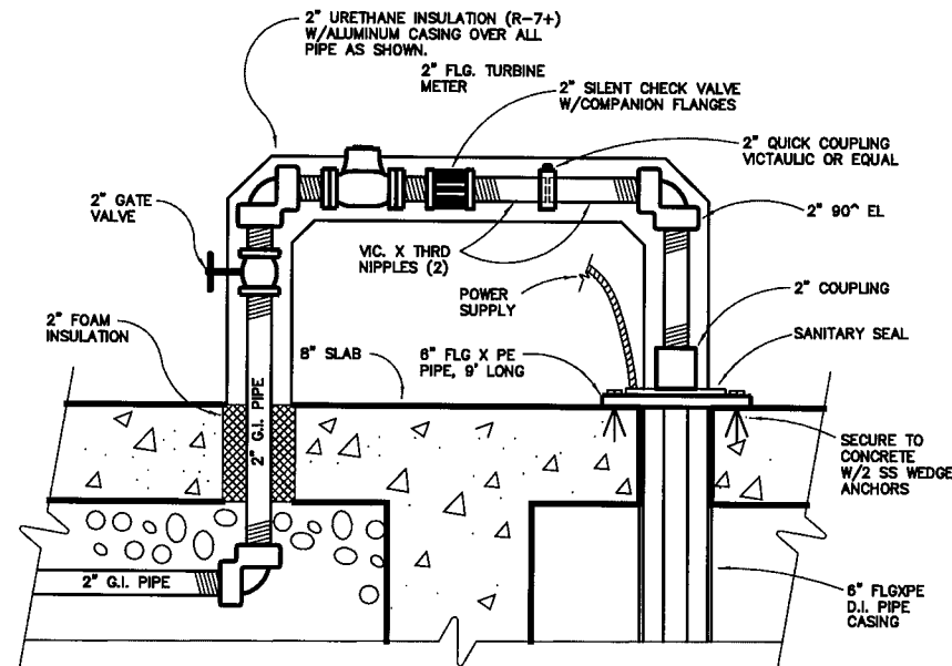
4 PROCESS WATER PIPING DETAIL NTS
