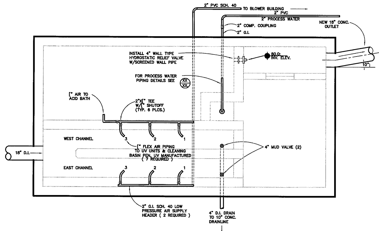
2 UV BASIN PIPING DETAILS SCALE: 1" = 1' - 0"
