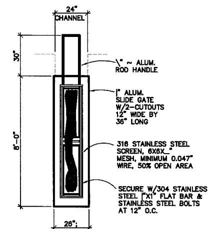
5 SCREENING GATE NTS (DETAIL FOR 15)
