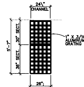
4 BAR SCREEN GATE NTS (DETAIL FOR 13, 14)
