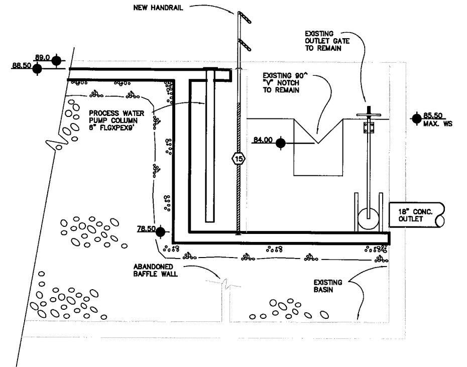
3 UV BASIN SECTION SCALE: 1" = 1' - 0"
