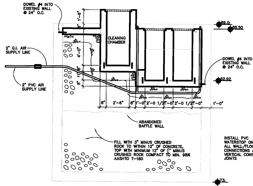
1 UV BASIN SECTION SCALE: 1" = 1' - 0"
