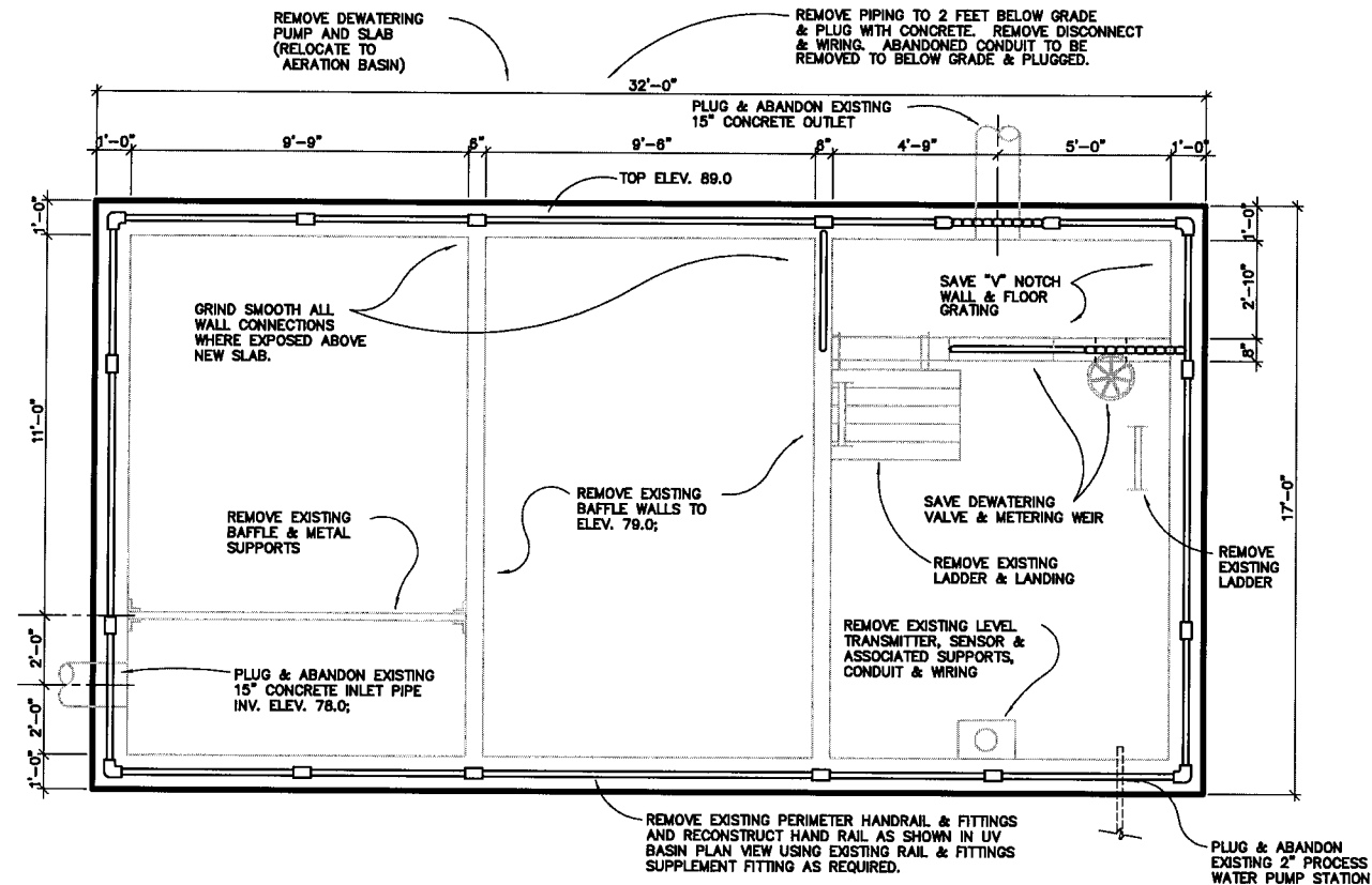
1 CHLORINE CONTACT CHAMBER DEMOLITION PLAN SCALE: 1" = 1' - 0"
