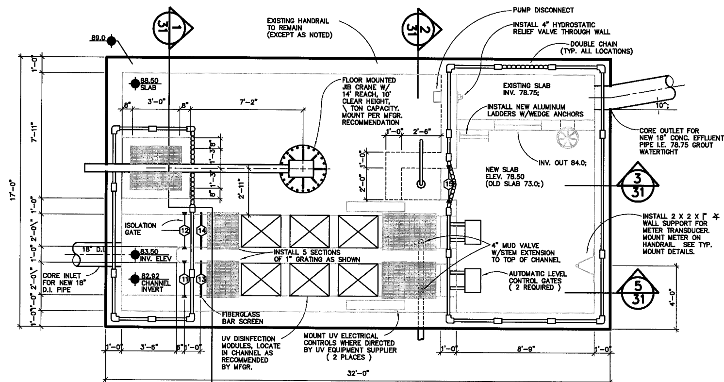
3 UV BASIN PLAN SCALE: 1" = 1' - 0"
