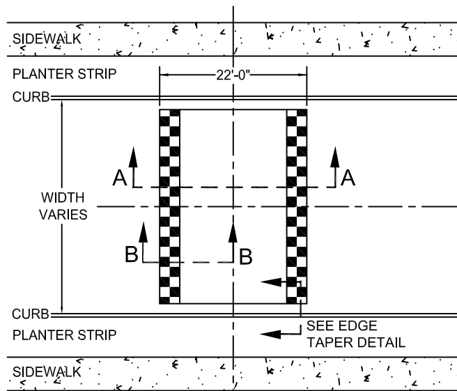
PLAN VIEW
