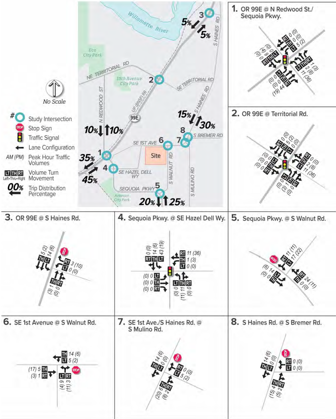
FIGURE 4: DISTRIBUTION OF SITE GENERATED TRIPS
