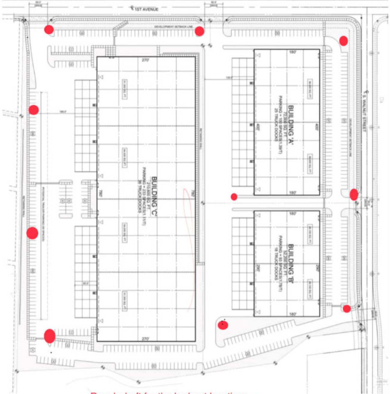
FIGURE 3: SITE PLAN
