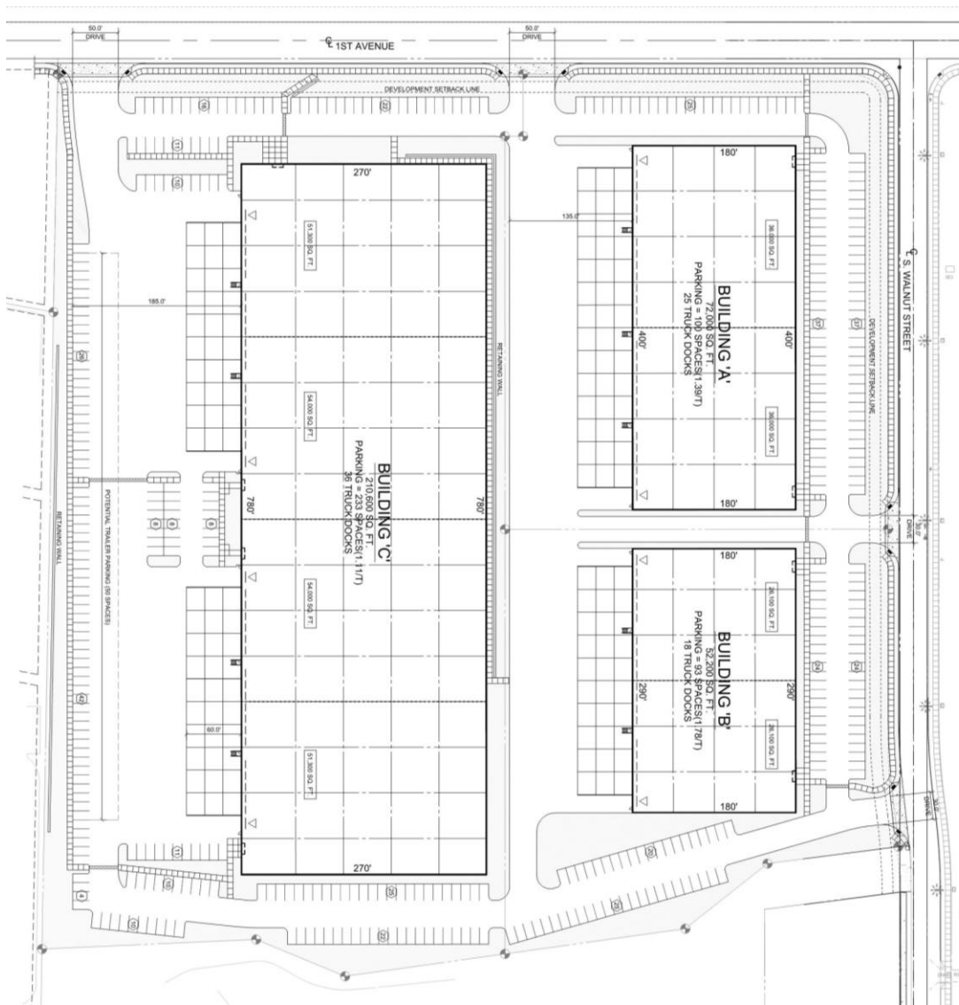
FIGURE 3: SITE PLAN
