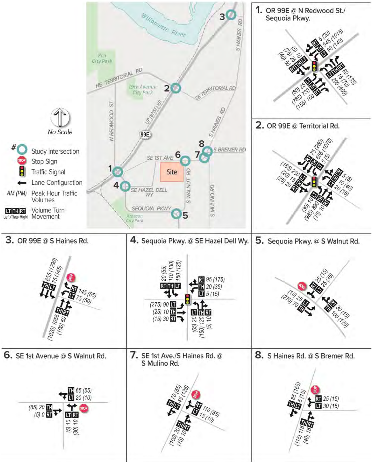
FIGURE 6: 2022 PROJECT CONDITIONS TRAFFIC VOLUMES
