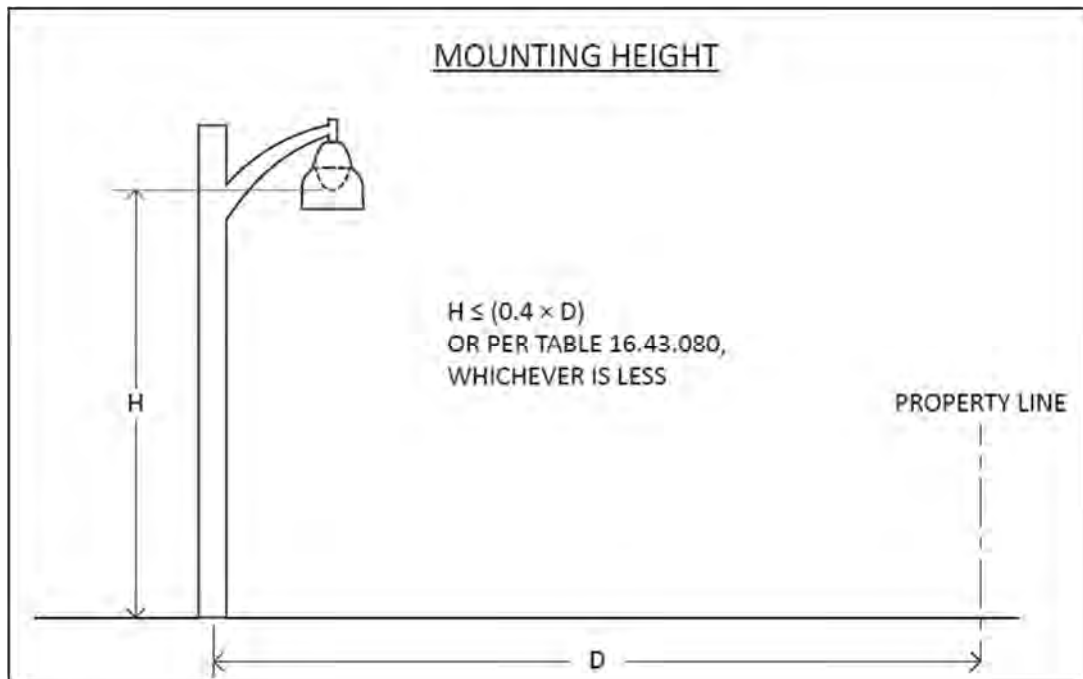
FIGURE 16.43.2: MOUNTING HEIGHT
