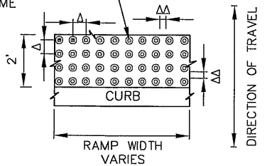
TRUNCATED DOME PATTERN AND ORIENTATION
