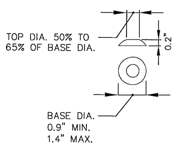
TRUNCATED DOME DETAIL
