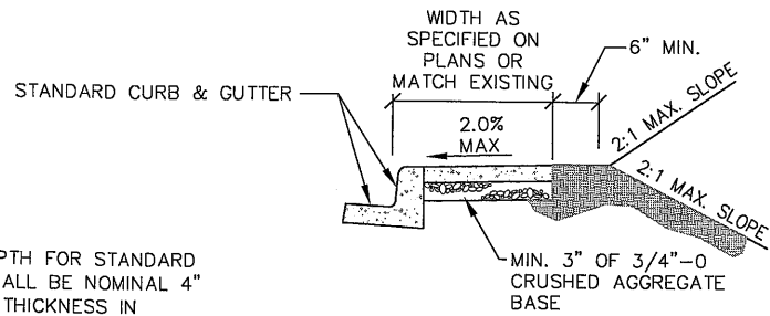
TYPICAL CURB TIGHT SIDEWALK
