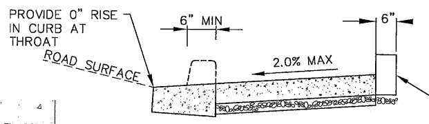
1 TYPICAL SIDEWALK DETAIL N.T.S.
