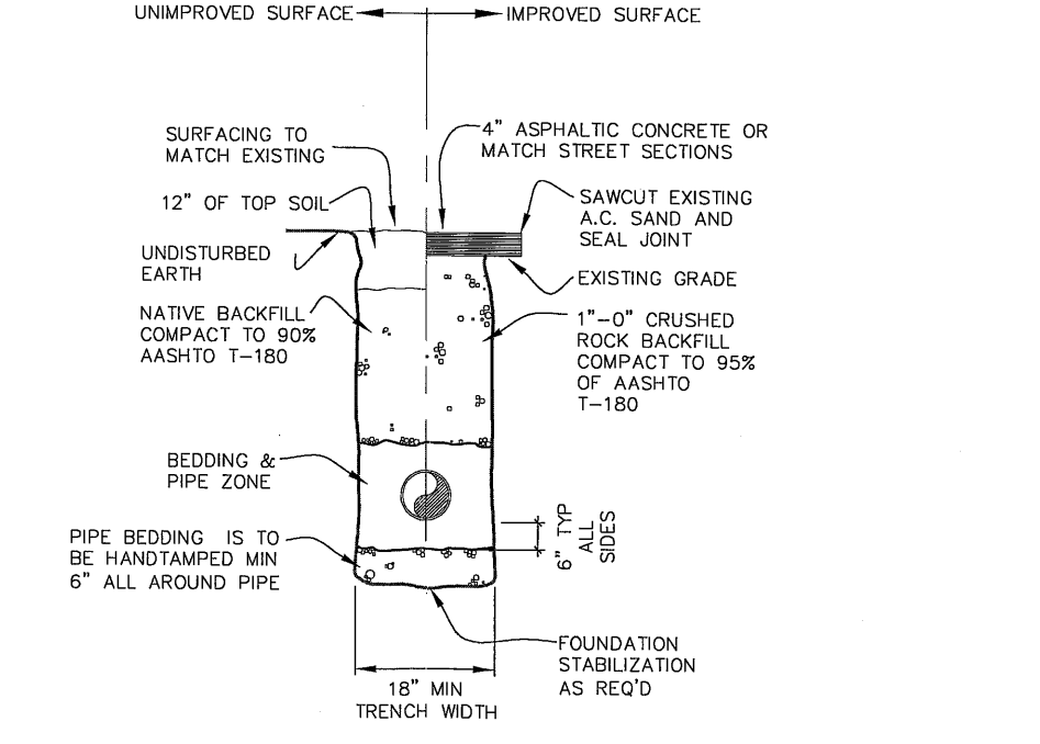
6 TYPICAL TRENCH DETAIL N.T.S.
